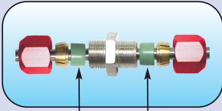
Refrigerant Leak Proof Seals
